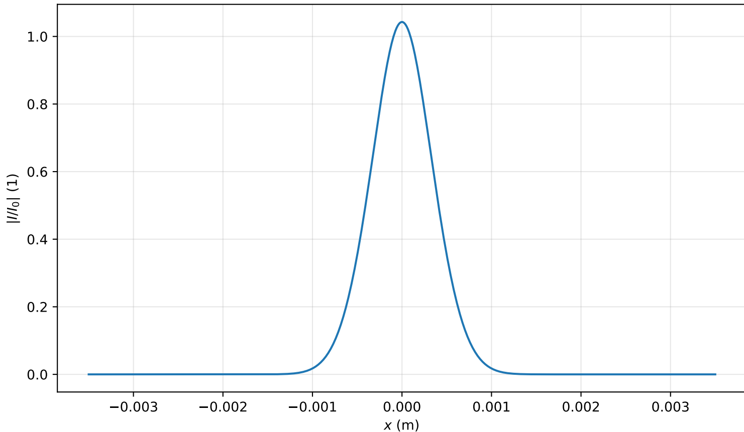
Intensity profile I(x, y = 0, z = 0.239m)/I_0 , P_{in}=1.0P_{cr} , artificial time
